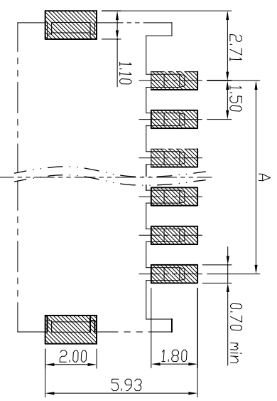
Recommended P.C.Board Layout (top view)
