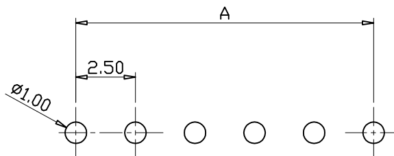
Recommended P.C. Board Hole Layout
