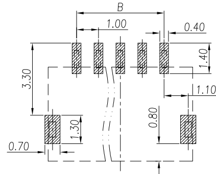
RECOMMENDED P.C. BOARD LAYOUT(TOP VIEW) GENERAL TOLERANCE : ±0.05
