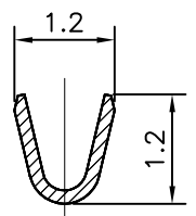
SECT. B-B
