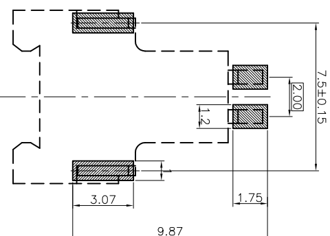
RECOMMENDED P.C. BOARD LAYOUT(TOP VIEW) GENERAL TOLERANCE : ±0.05
