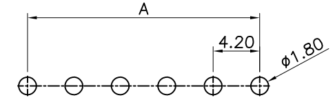
Recommended P.C.Board Hole Layout
