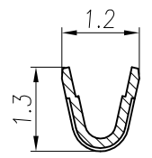
SECT. A-A
