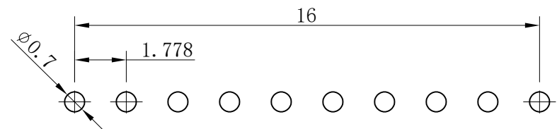
Recommended P.C.Board Hole Layout
